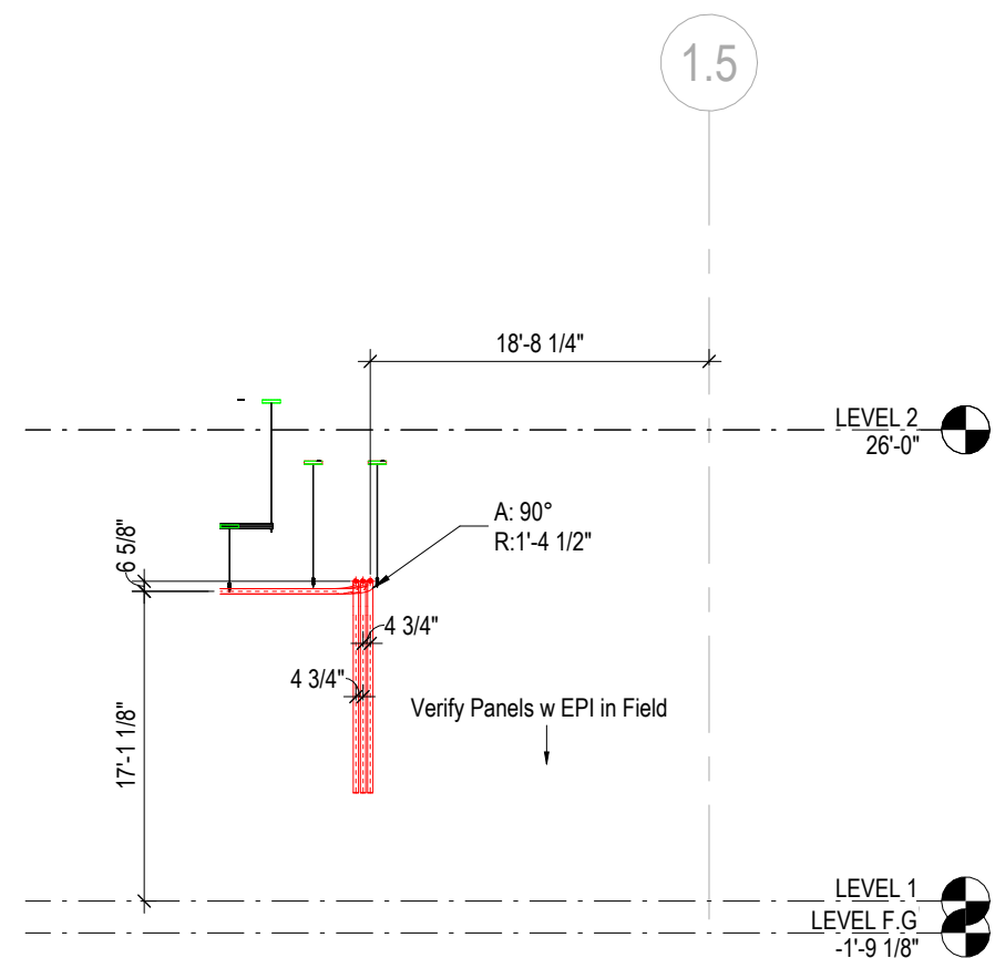
③ H71-01-A3-S2 3/32" = 1'-0"
